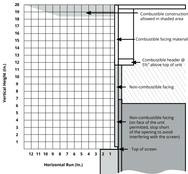
Figure 3. Non-combustible mantles and facings.
