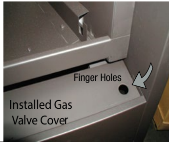
Figure 7. Removing and installing the Horizontal Access Panel
